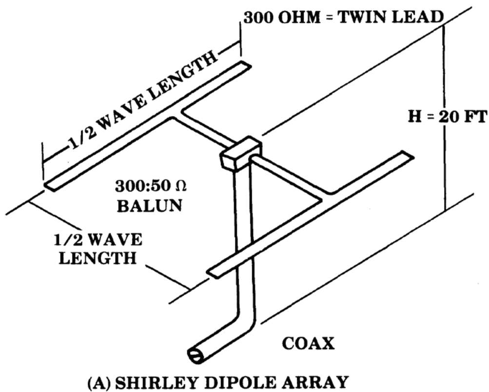
Figure M-7. The Shirley Dipole
