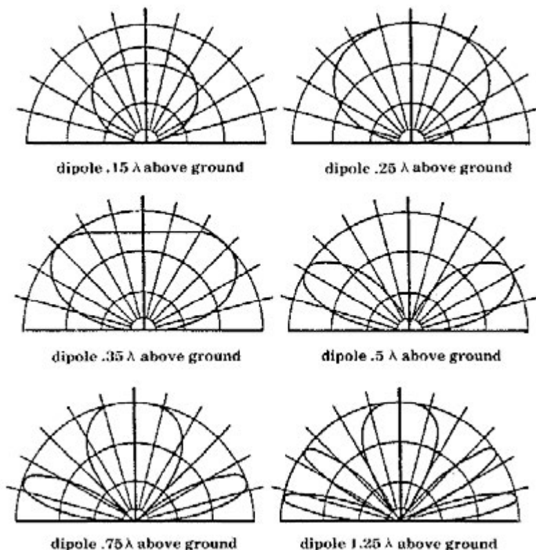
Figure 3. Horizontal dipole radiation patterns at various heights (in wavelengths) above the ground (from Air Force Comm. Pam. 100-16).
