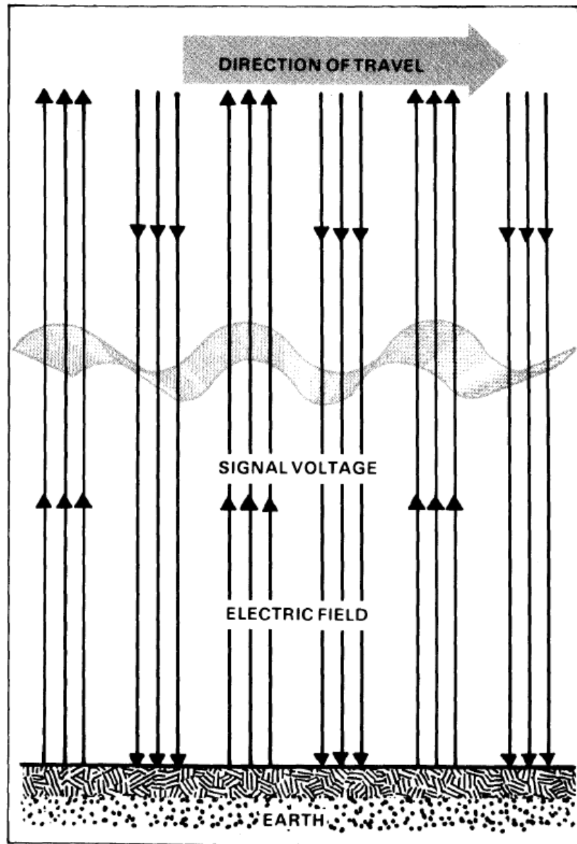
Figure 3-4. Vertically polarized signal.
