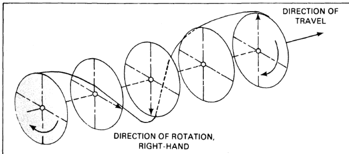
Figure 3-6. Circular polarized wave.
