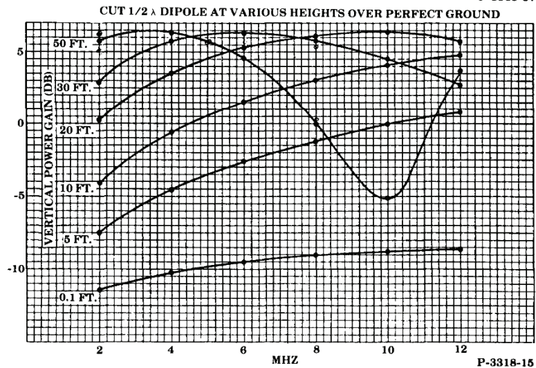
Figure 2. CUT \frac{1}{2} \lambda DIPOLE AT VARIOUS HEIGHTS OVER AVERAGE GROUND
