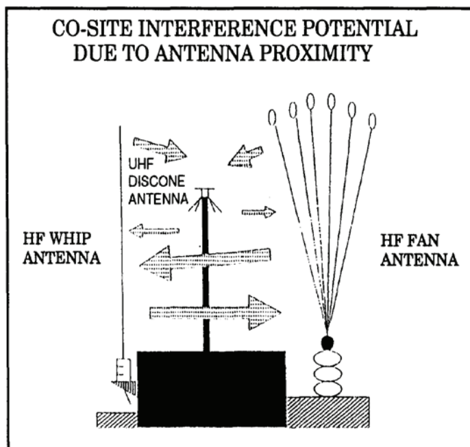
Figure 11. Electromagnetic co-site problems caused by Antenna Proximity
