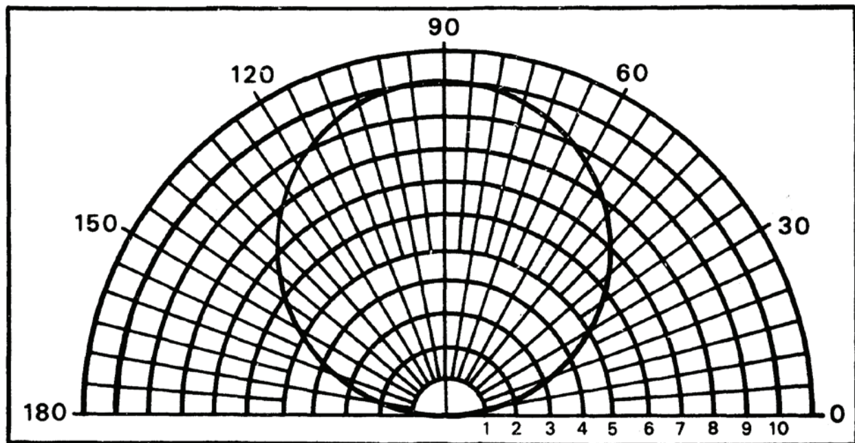
Figure M-4. Typical elevation plane pattern.
