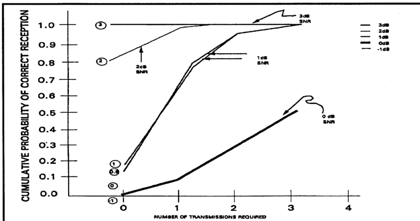
Figure 7. System improvements resulting from use of AN/PSC-2 digital communications terminal. With 3dB SNR, message was received every time. Requires a 10dbB SNR.
