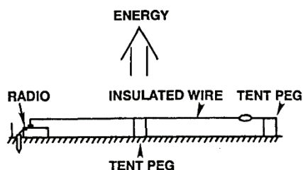
Figure 2. Simple wire antenna for low power radio. (Height can be from a few inches to 30 feet. Do not let wire contact ground. Use more pegs to keep wire off ground if needed.)
