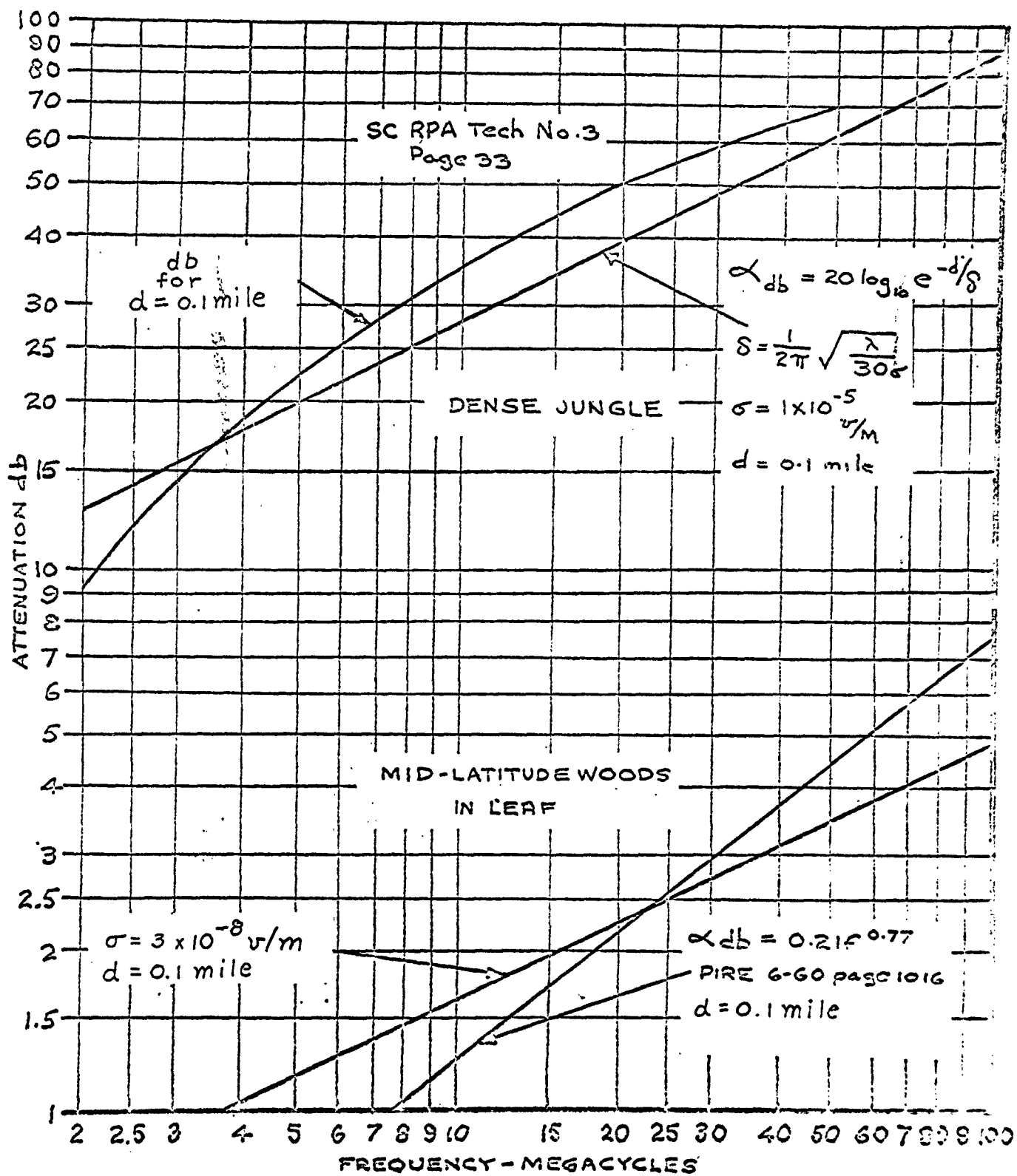
Figure 1. Radio Wave Attenuation Through Jungle and Woods
